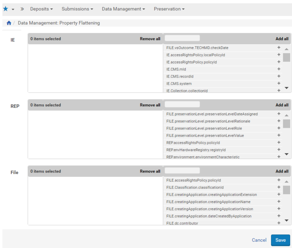
Figure 71: Property Flattening
