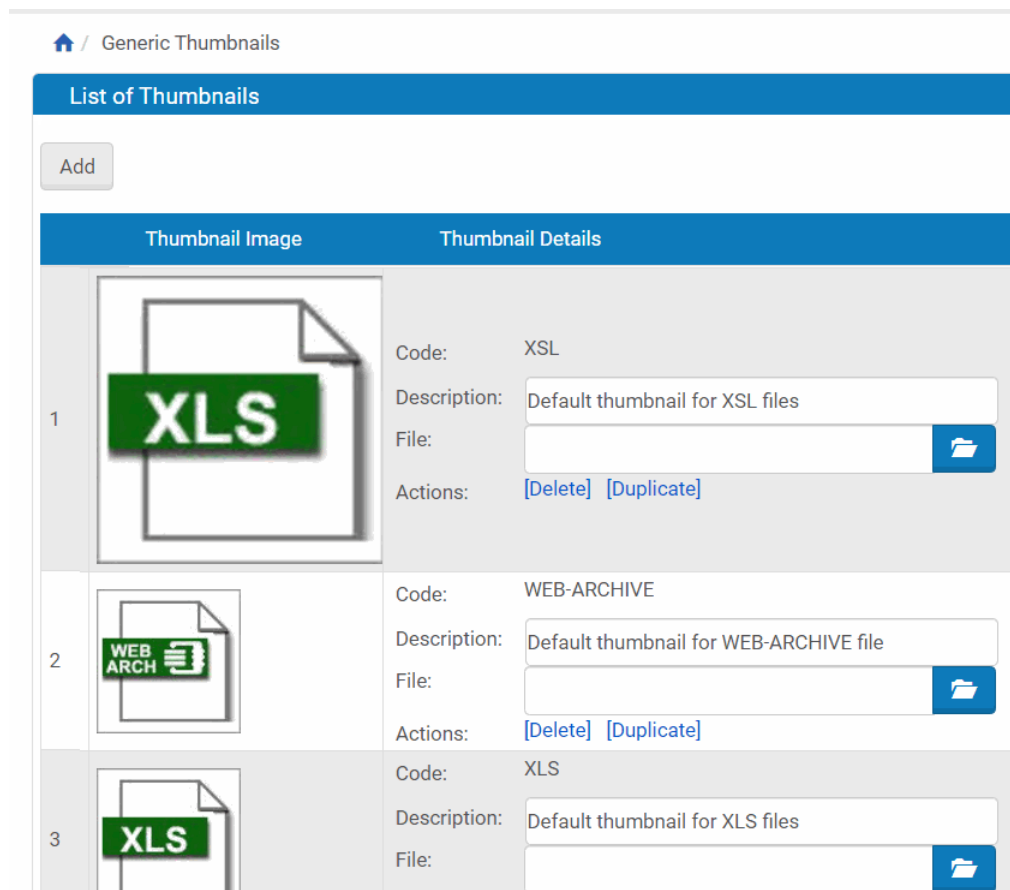
Figure 56: Generic Thumbnails
