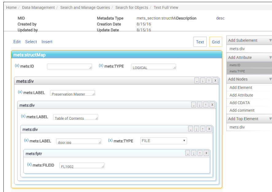
Figure 242: Add Structmap – Grid View
