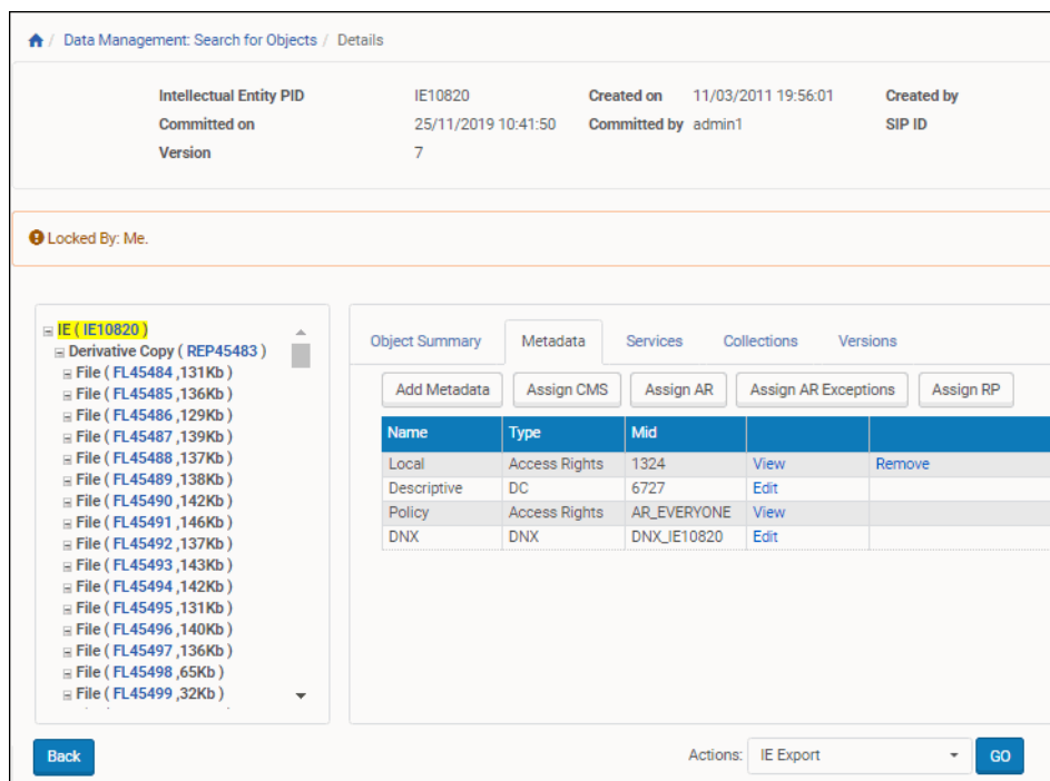
Figure 218: Web Editor - Metadata Tab
