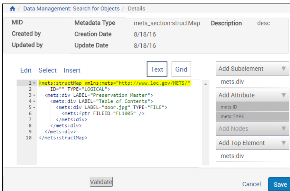
Figure 241: Add Structmap – Text View
