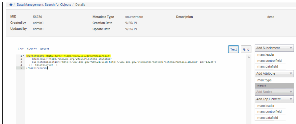
Figure 242: Text View
