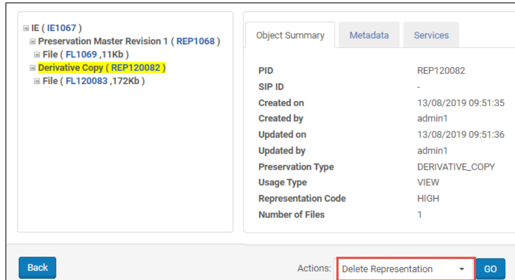
Figure 256: Delete Representation
