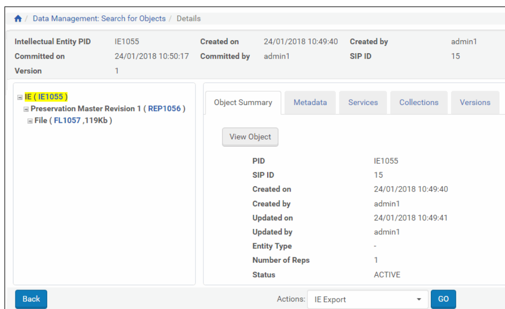
Figure 218: Web Editor
