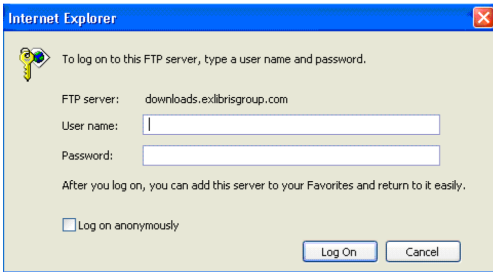
Figure 1-17. FTP Login
